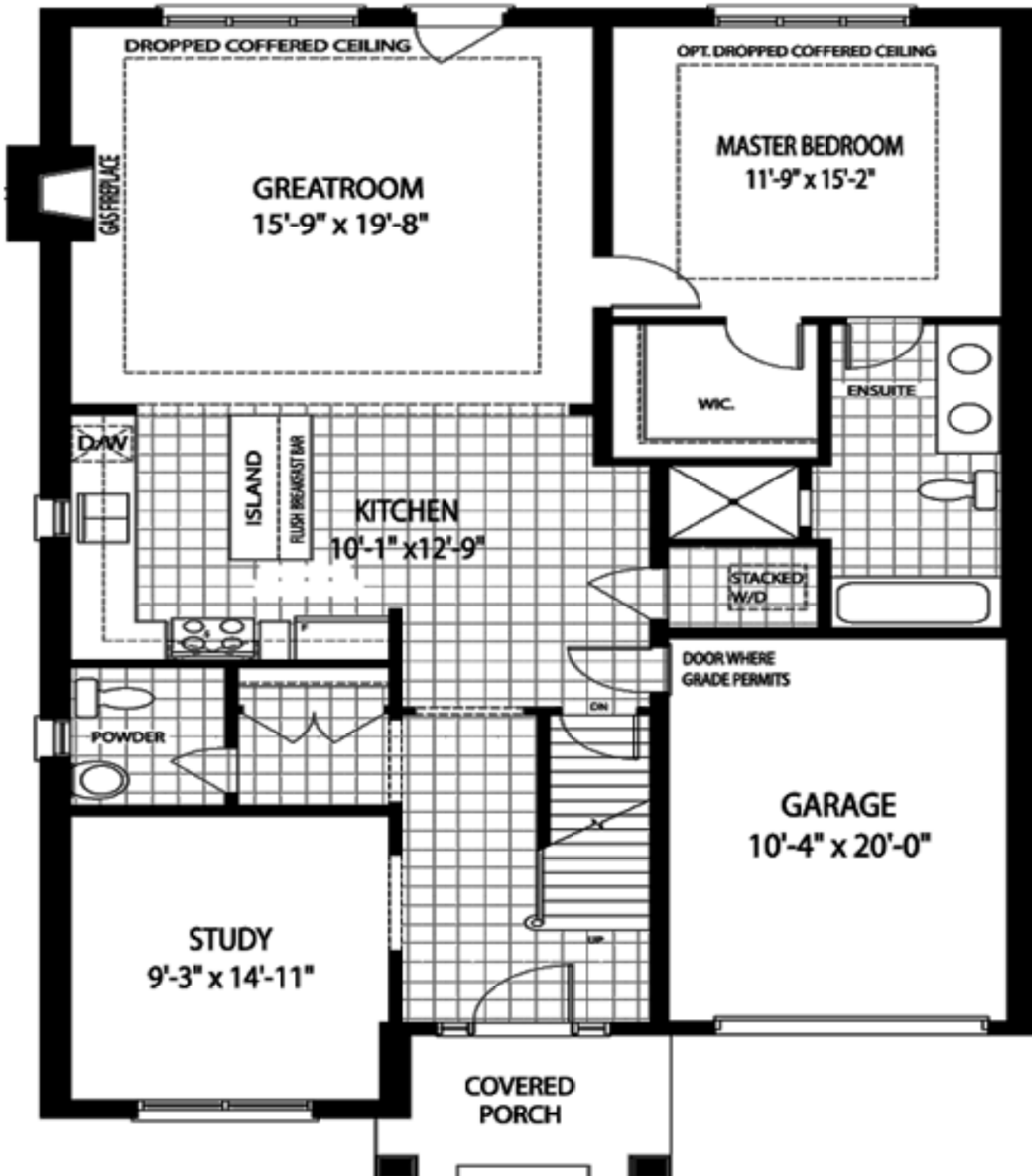
The Glencairn Ground Floor Plan A
