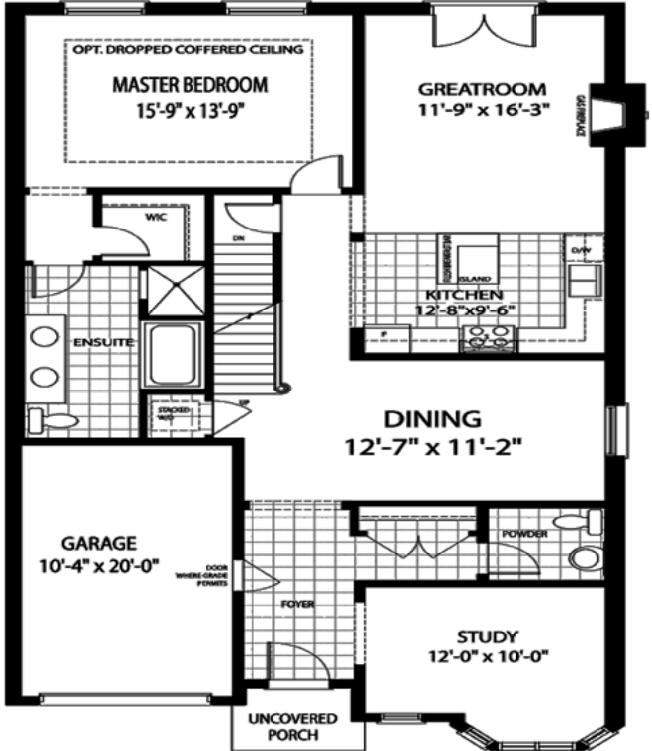
The Speyside Ground Floor Plan A
